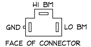
HEADLIGHT CONNECTORS
