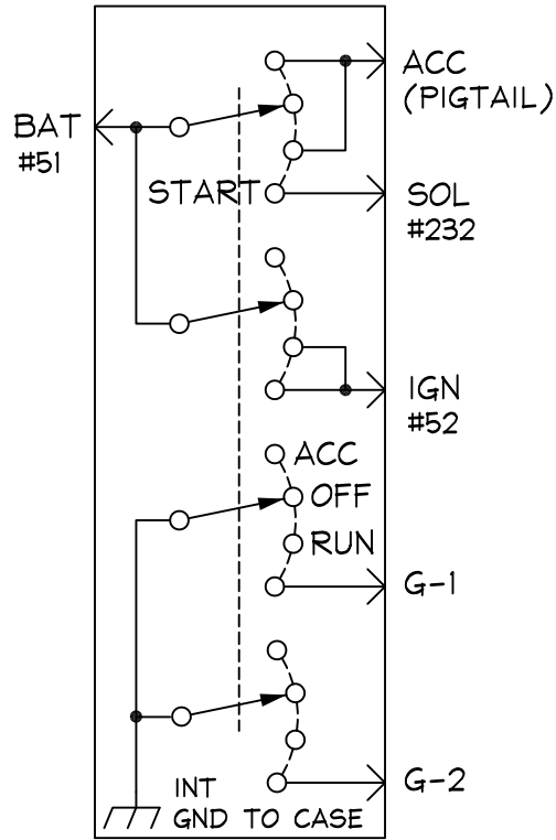
IGNITION SWITCH
