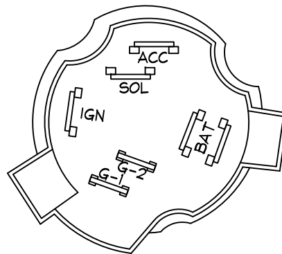
IGNITION SWITCH
