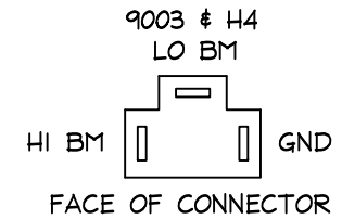
HEADLIGHT CONNECTORS
